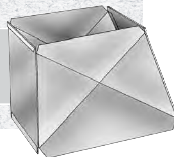
#411 End Cap
