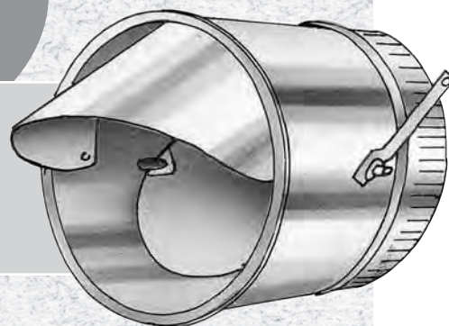
#703 Spin-In with scoop & damper
