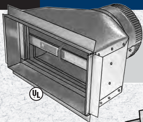
#500RD Ceiling Radiation Damper Sleeve
