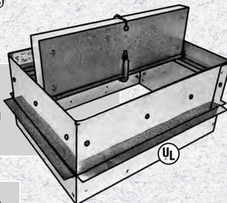
#500RD Ceiling Radiation Damper Sleeve
