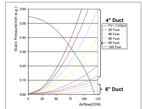
FV-11VQL6 110 CFM 4" or 6" Duct
