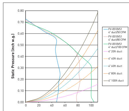
FV-0510VS1 50-80-100 CFM 4" Oval Duct
