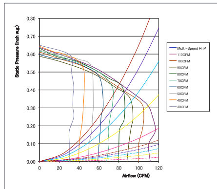
FV-05-11VKL1 50-80-110 CFM 4" or 6" Duct
