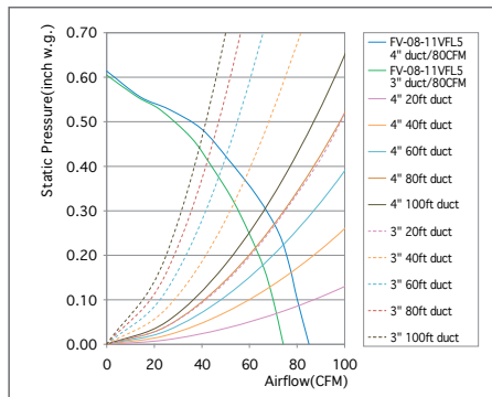
FV-08-11VFL5 80 CFM 4" or 3" Duct
