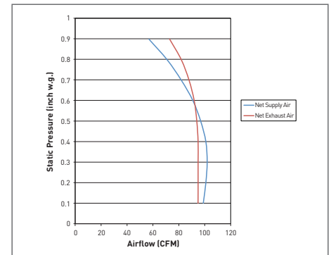
FV-10VE1 50-80-100 CFM 4 x 4" or 6" Ducts
