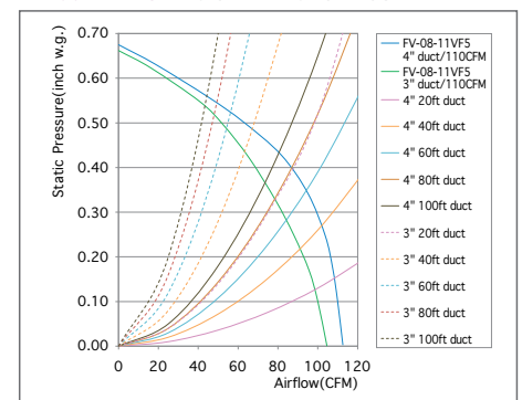
FV-08-11VF5 110 CFM 4" or 3" Duct
