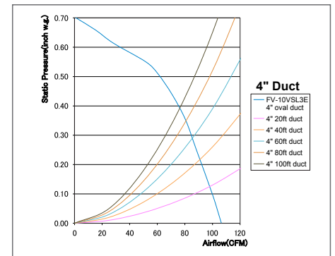
FV-10VSL3E 100 CFM 4" Oval Duct
