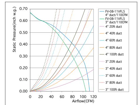
FV-08-11VFL5 110 CFM 4" or 3" Duct
