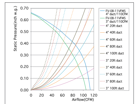
FV-08-11VFM5 110 CFM 4" or 3" Duct
