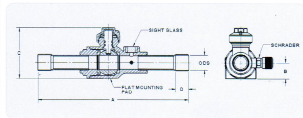
BALL VALVES WITH SIGHT GLASS & MOISTURE INDICATOR
